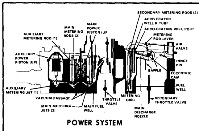
Figure 21 Multiple Stage Power System
