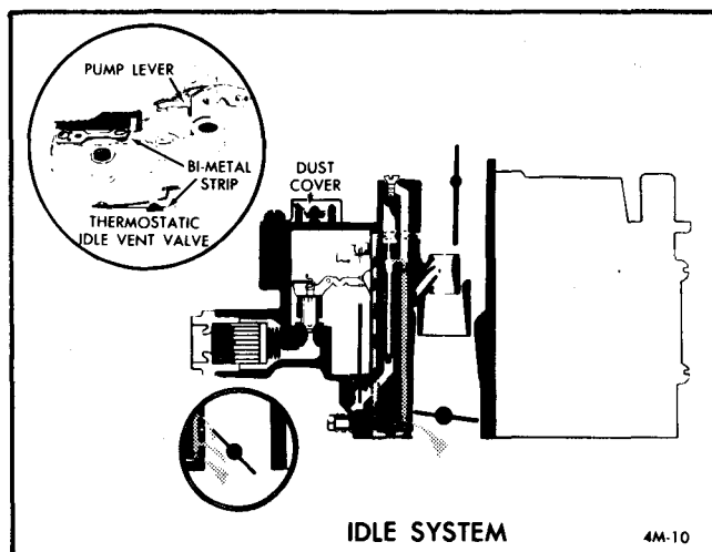
Figure 8 Thermostatic Idle Vent Valve
