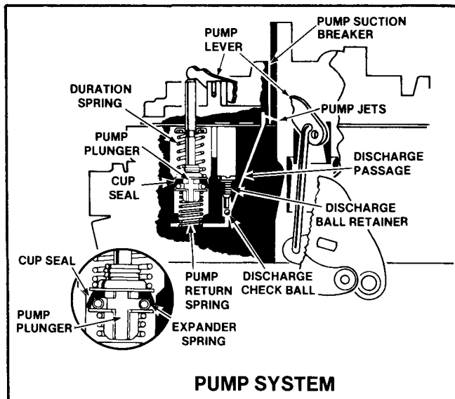
Figure 24 Pump System
