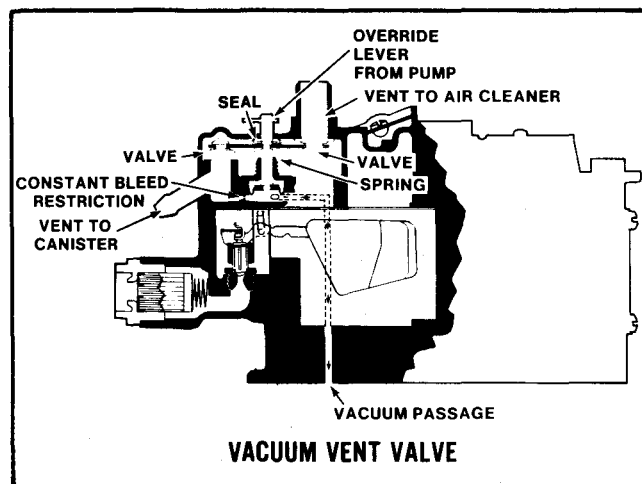
Figure 9 Bowl Vent Valve
