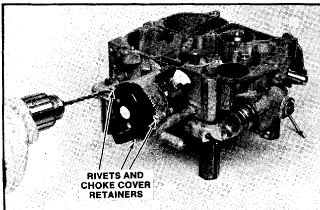
Figure 59 Choke Cover Removal - Late Models
