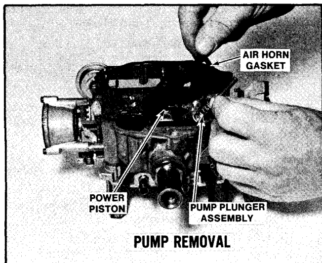
Figure 49 Pump Removal
