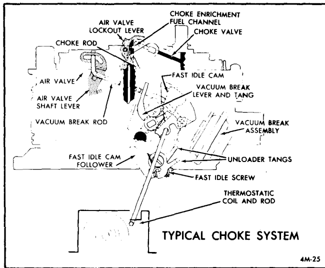
Figure 26 Choke System-4MV
