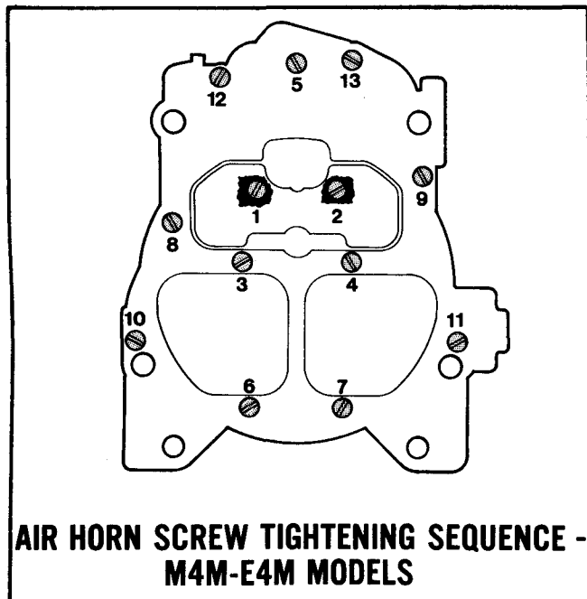
Figure 70 Air Horn Screw Tightening Sequence
